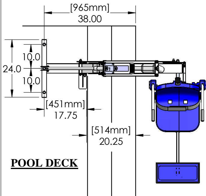
PLAN VIEW PRO POOL-XR ON TYP. CURB
