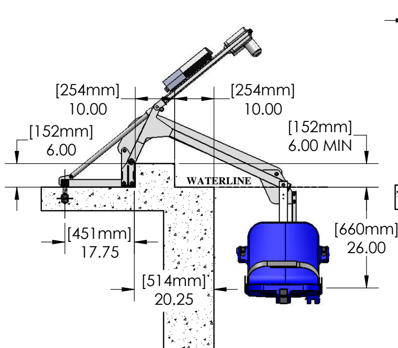
SIDE VIEW PRO POOL-XR ON TYP. CURB
